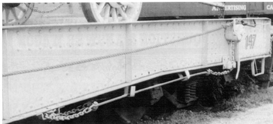
Brake & Rod Set-up
