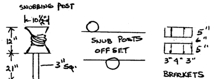
Snubbing Post
